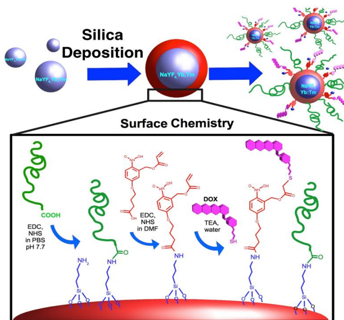
Scheme 3.3. Schematic representation of the surface modification of the silica-coated UCNPs, which yields PEG- and Dox-functionalized UCNPs@SiO 2 nanoparticles.
