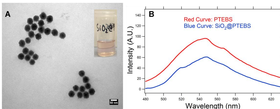
Figure 6.5. A) TEM micrograph of the \text{SiO}_2\text{@PTEBS} nanoparticles. Scale bar is 50 nm. The inset is a picture taken from the vial containing the nanoparticles. B) Photoluminescence of the original PTEBS polymer (red curve) and the PTEBS encapsulated in the silica nanoparticles (blue curve). The excitation wavelength was 420 nm.
