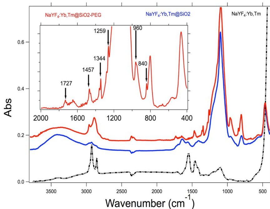
Figure 6.17. FTIR spectra of NaYF 4 :Yb,Tm (dotted black line), NaYF 4 :Yb,Tm@SiO 2 (blue line) and NaYF 4 :Yb,Tm@SiO 2 -PEG (red line). The inset depicts a magnification of NaYF 4 :Yb,Tm@SiO 2 -PEG spectra in the region comprised between 2000 and 400 \text{cm}^{-1} .
