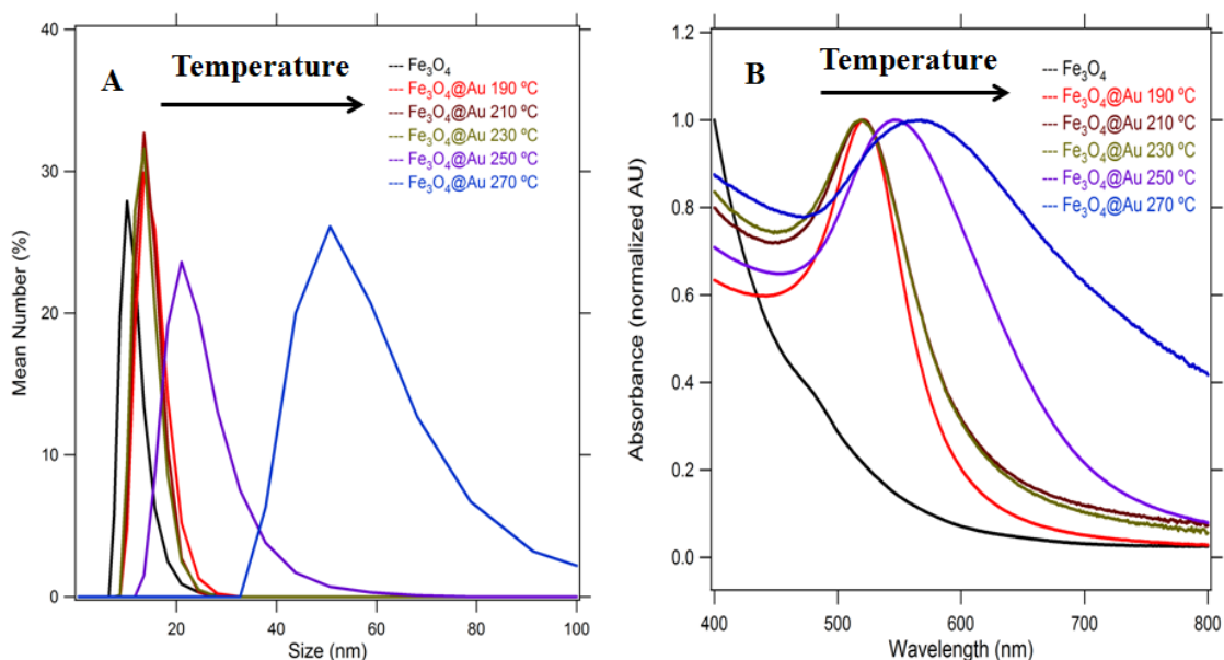
Figure 5.9. a) Size distribution obtained by DLS of the \text{Fe}_3\text{O}_4 @Au nanoparticles synthesized at different reaction temperatures. b) UV-Vis spectra of the \text{Fe}_3\text{O}_4 @Au nanoparticles synthesized at different reaction temperatures.
