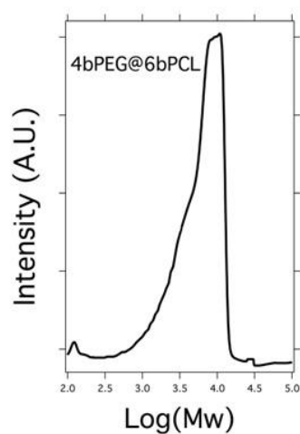
Figure 4.7. GPC curve of the 4bPEG@6bPCL polymer.
