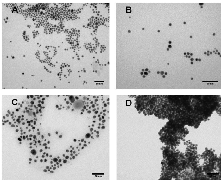
Figure 5.8. TEM micrographs from the \text{Fe}_3\text{O}_4 @Au nanoparticles synthesized at different reaction temperatures: a) 210 °C b) 230 °C c) 250 °C and d) 270 °C.
