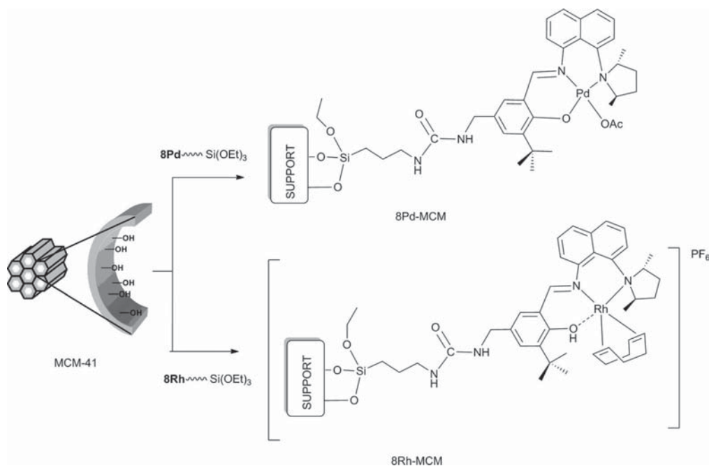
Scheme 4 Heterogenization of imino complexes.
