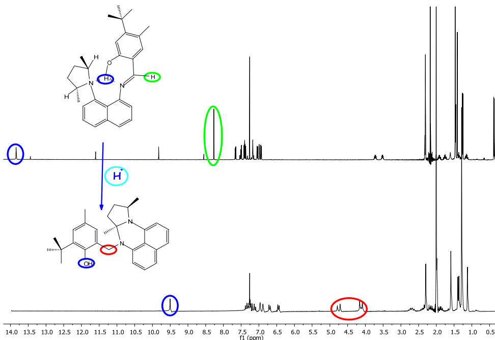
Figure. IV. 24. 1 H-NMR spectrum of (R,R)-8 before (up) and after (down) acid treatment.
