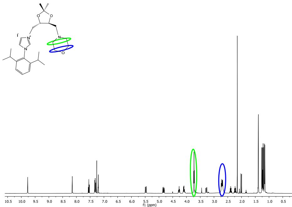
Figure. III. 25. 1 H NMR spectrum for ( S,S )- [4b]I
