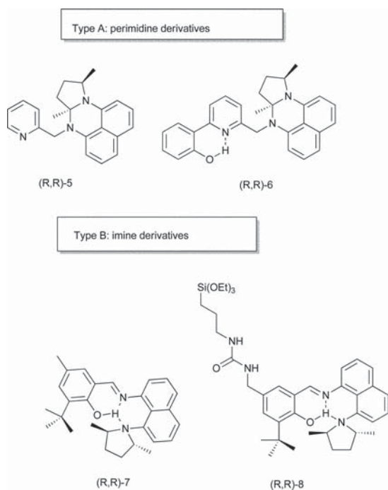
Fig. 1 Chiral perimidino and imine ligands.
