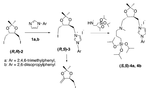
Scheme 1. Synthesis of chiral mono-NHC ligand precursor.
