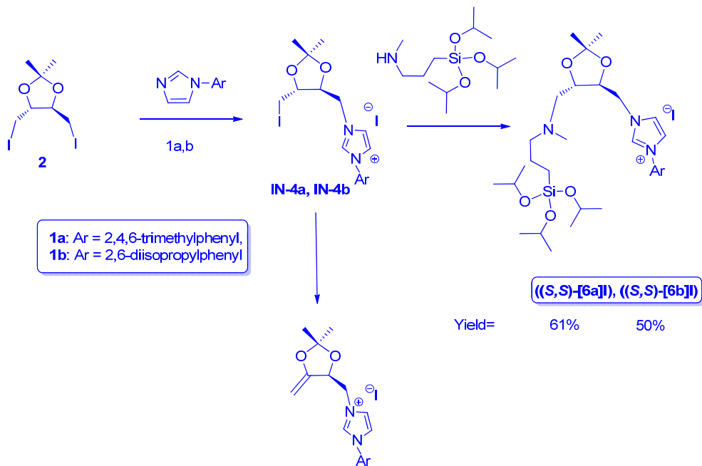
Figure. III. 26. Synthesis of mono -NHC amine precursor salts with pendant alkoxy silane groups.
