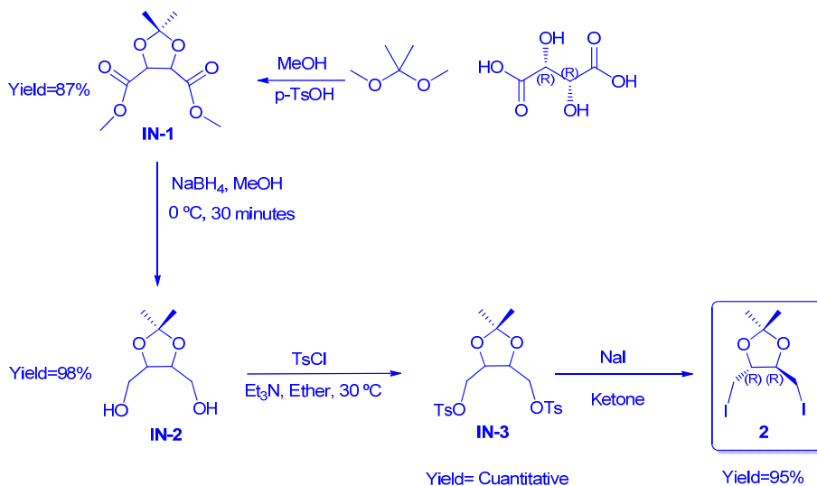
Figure. III. 18. Synthesis of dioxolane chiral backbone.
