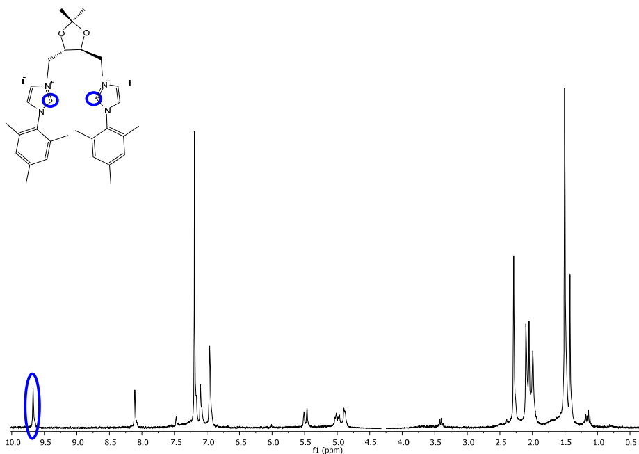
Figure. III. 21. 1 H NMR spectrum for ( S,S )- [3a]I .
