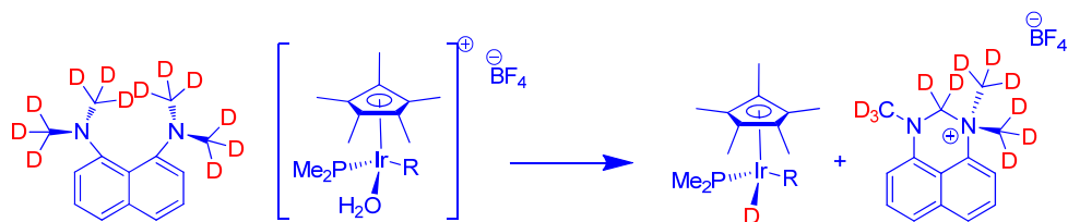
Figure. IV. 11. Hydride transfer in Iridium complex.
