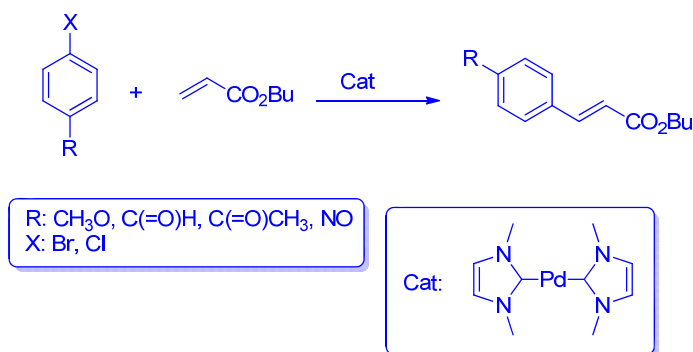
Figure. III. 10. First example of NHC catalytic properties in Heck reaction.
