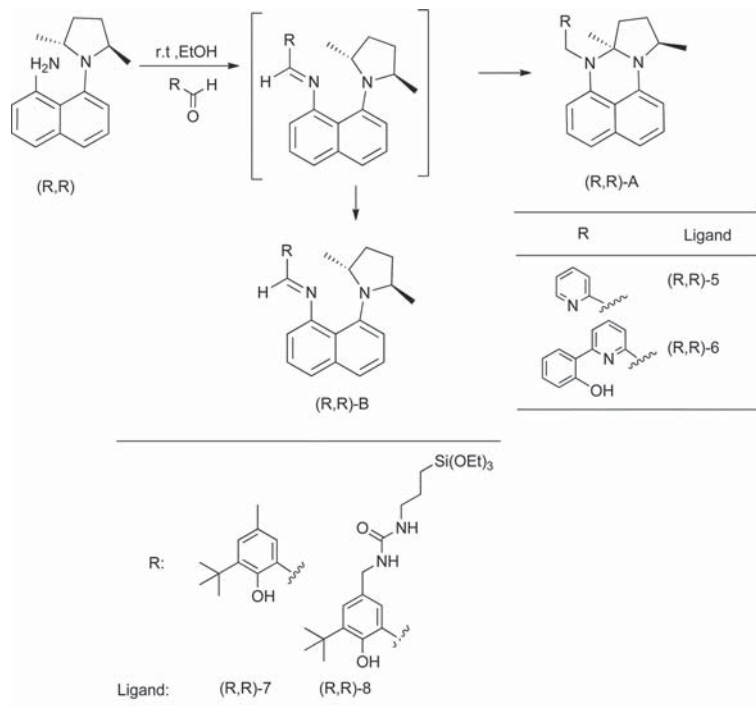
Scheme 1 Condensation products of 8-(( R,R )-2,5-dimethylpyrrolidin-1-yl)naphthalen-1-amine with different aldehydes.
