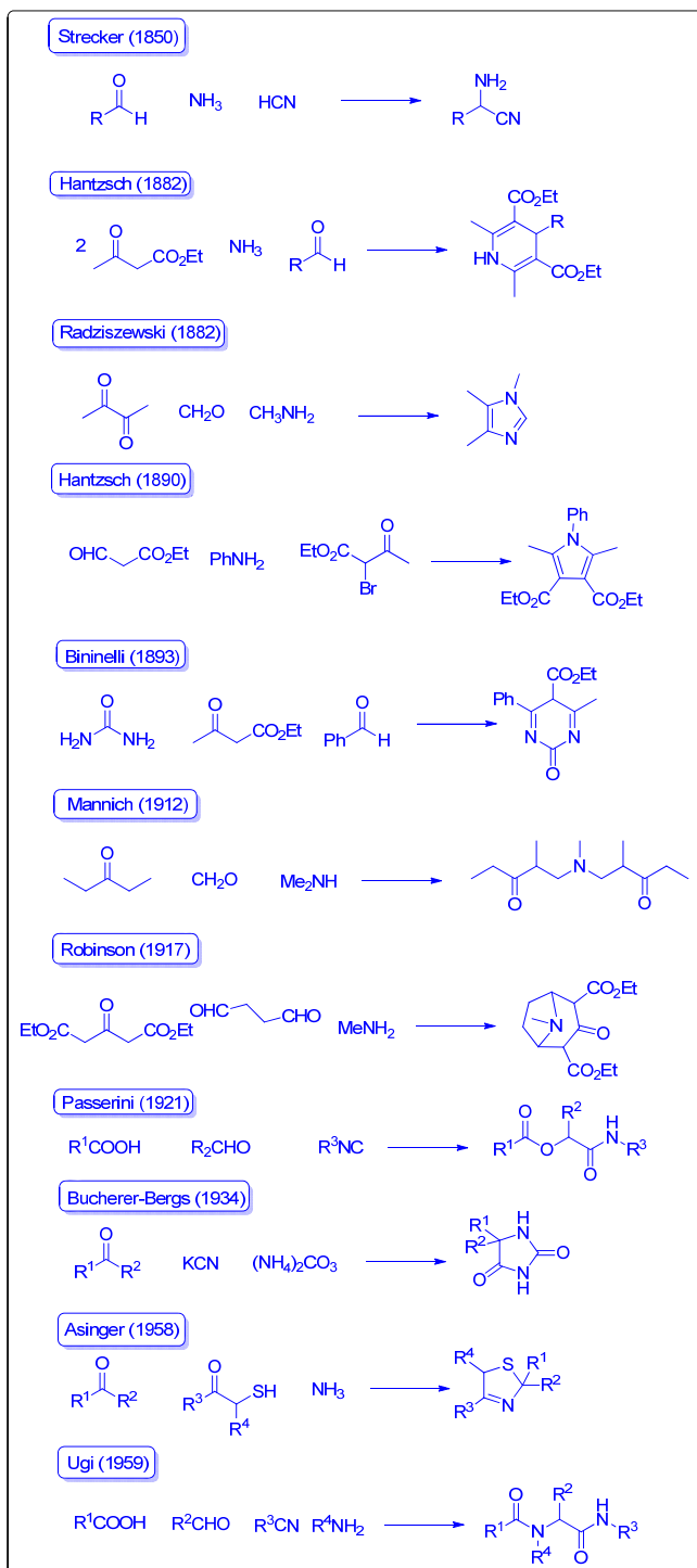
Figure. V. 2. Historical background of MCR's.
