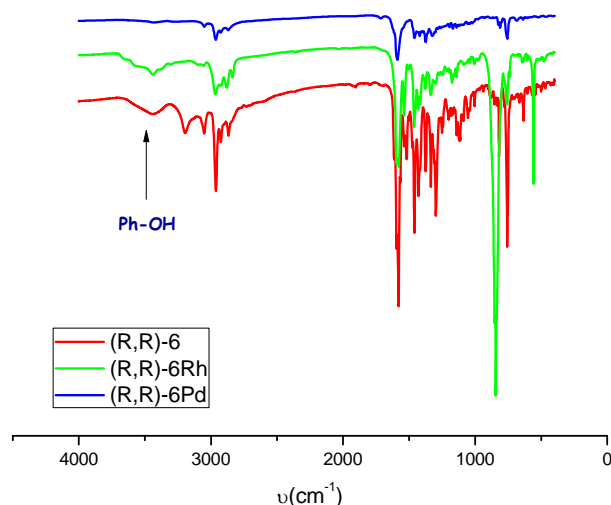
Figure. IV. 26. IR of (R,R)-6 and its rhodium and palladium complexes.
