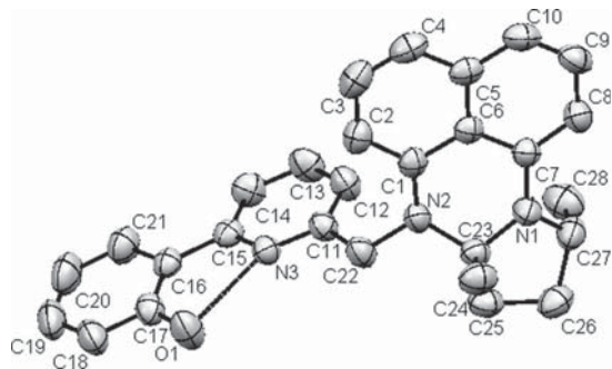
Fig. 2 Molecular structure of ( R,R )- 6 .
