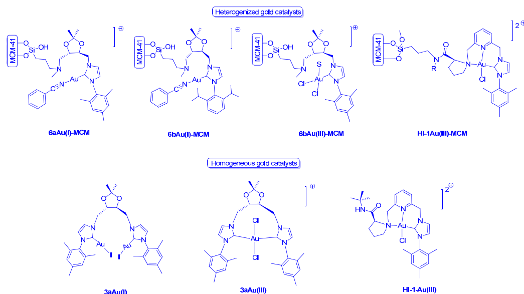
Figure. V. 10. Supported and soluble gold (I) and gold (III) catalysts.
