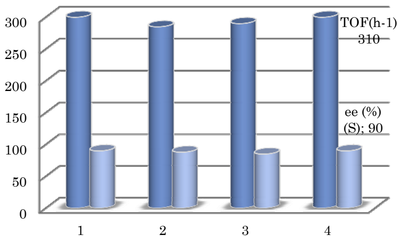
Figure. IV. 38. Recycling of 9Rh-MCM .
