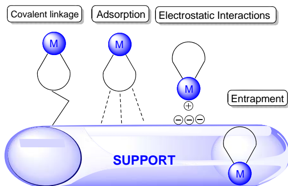
Figure. I. 6. Strategies for immobilizing soluble catalyst on solids.
