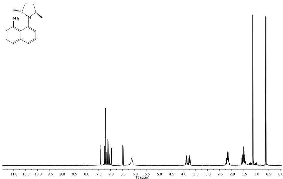
Figure. IV. 16. 1 H-NMR spectrum of ( R,R )-4.
