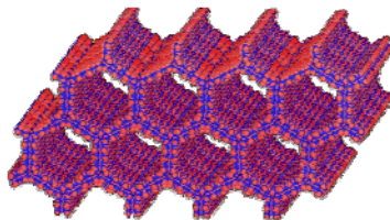
Figure. I. 5. MCM-41 structure.
