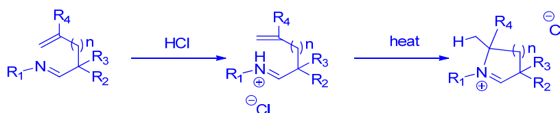
Figure. III. 7. Intramolecular quaternization of imines.
