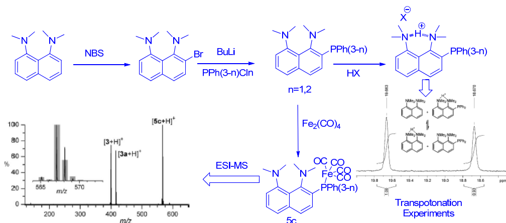
Figure. IV. 10. Useful metallation of phosphine-DMAN.
