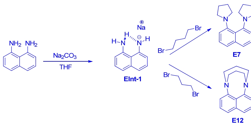
Figure. IV. 5. Synthesis of cyclized amine naphthalene PS's.
