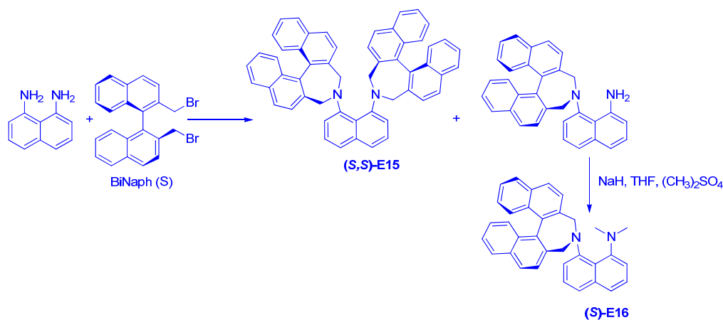
Figure. IV. 9. First chiral atropisomer PS.
