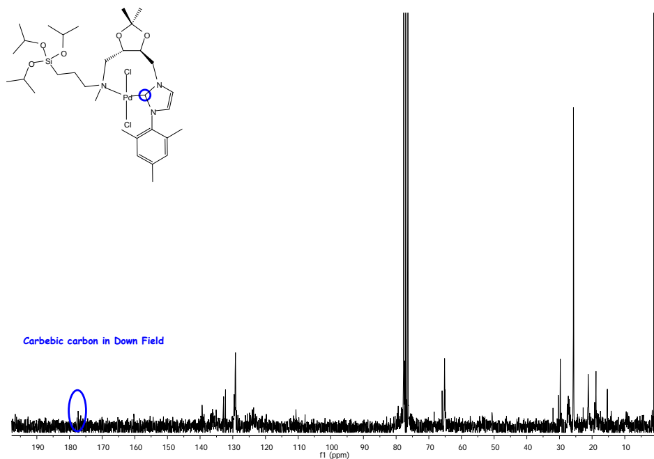
Figure. III. 33. ^{13}\text{C} NMR spectrum for ( S,S )- 6aPd .
