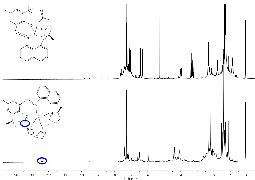
Figure. IV. 30. 1 H-NMR spectrum of (R,R)-8Pd (deprotonated) and (R,R)-8Rh (protonated).
