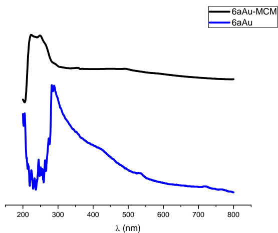
Figure. III. 38. Uv-Vis and DFTR spectrum (S,S) - 6aAu(I) before and after heterogeneization.
