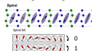
Spin-induced multiferroics
