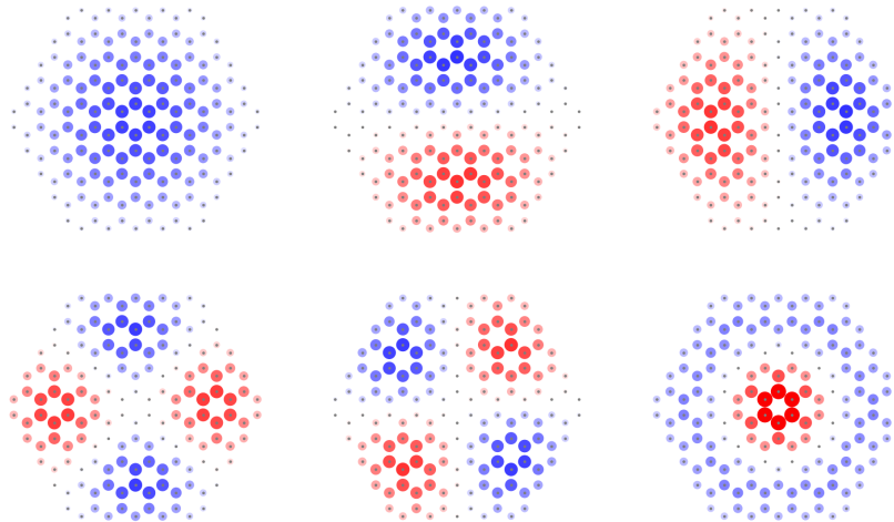
Fig. Field distributions in selected eigenmodes in a hexagonal waveguide array.
