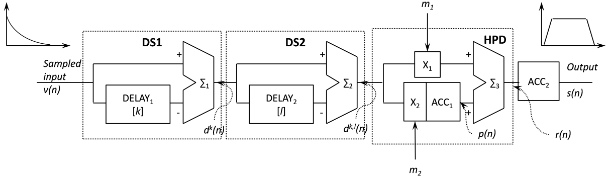
Figure 4. Diagram of the digital trapezoidal shaper. The elements are: \text{DELAY}_n - a delay pipeline, \Sigma_n an adder/subtractor, \text{ACC}_n an accumulator, X_n a multiplier. \text{DS}_n is a delay-subtractor unit, HPD is a high-pass filter deconvolver.
