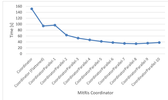
Figure 8. Performance comparison of xDEVS Coordinators.
