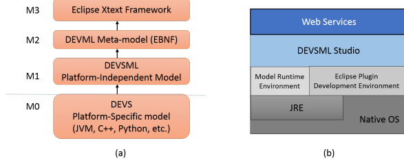
Figure 3. (a) Metamodeling layers and (b) DEV SML Studio software architecture.
