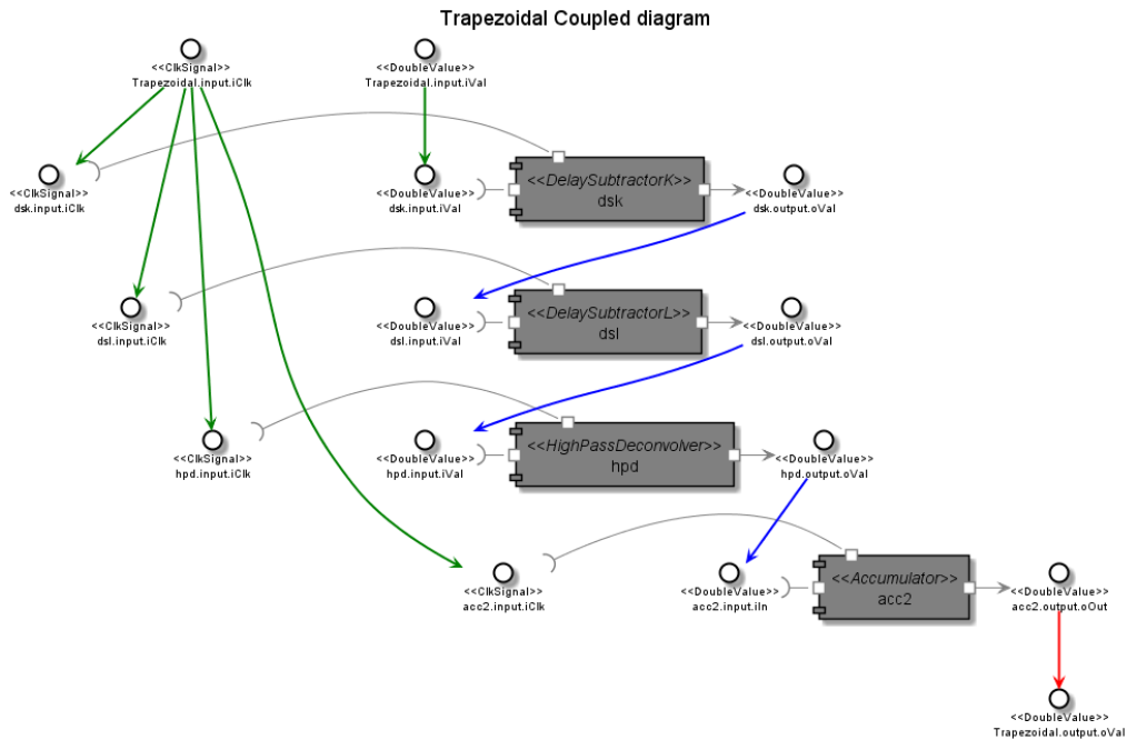
Figure 6. Auto-generated Coupled model representation with port data-types. Green arrows represent External Input Coupling (EIC), blue arrows represent Internal Coupling (IC), and red arrows represent External Output Coupling (EOC).
