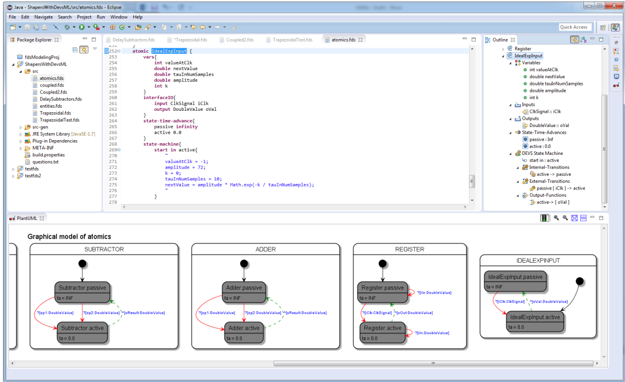
Figure 5. DEVSML Studio showing auto-generated DEVS Atomic visual and hierarchical representation.
