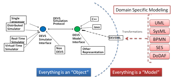
Figure 1. Integrating theory of modeling and simulation framework with MDE [22].
