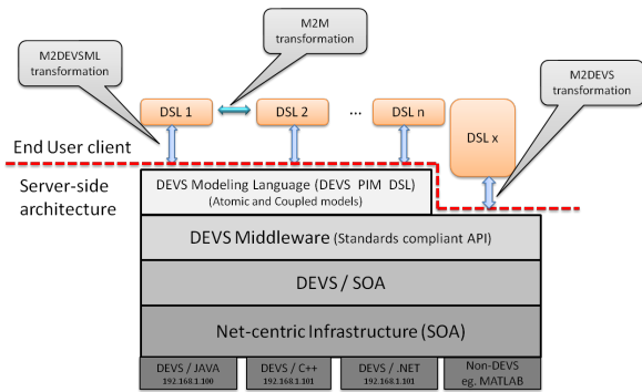
Figure 2. DEVSML Stack showing DEVS modeling language and various transformations [19].
