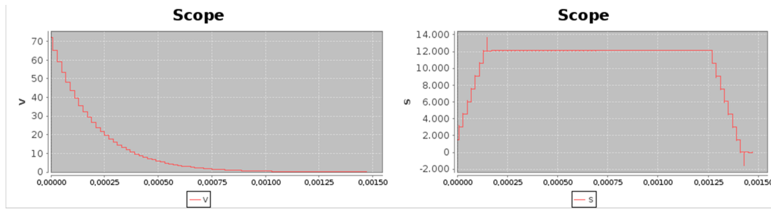
Figure 7. Exponential input (left) and trapezoidal output (right) generated by the xDEVS shaper model for one single event.
