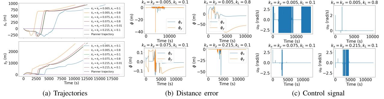
Figure 4: Controller testing for scenario A2.
