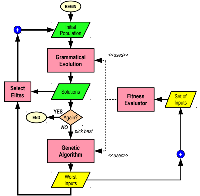
Figure 1: Optimization flow. Thick arrows represent the execution path, regular arrows indicate data transmission and dotted arrows indicate usage.
