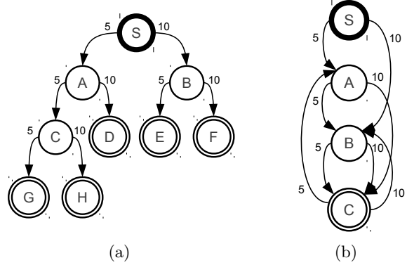
Figure 2: (a) FSM solving 15¢ vending machine. Transitions from the final states to S were removed. (b) Reduced FSM for the 15¢ vending machine.
