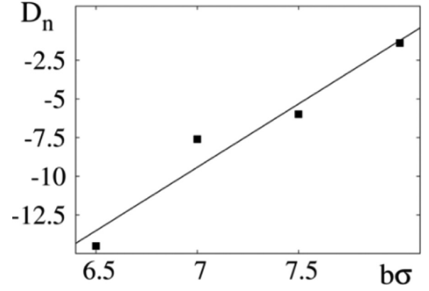
Fig. 7. Dependence of value \log(D_{n,cr}) on lattice stiffness b\sigma (dots) and its linear approximation f(x)=8.19x-66.7 (solid line).
