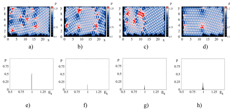
Fig. 8. Crystal-like triangular lattice. Translational mode after noise influence (from left to right – with different realizations of noise). Presented states correspond to local potential minimum; these defects are remaining in the lattice which translates in some direction "as a whole". Top panels: a)-d) spatial distribution of units. Bottom panels: e)-h) kinetic energy distribution p(E_k) (shows a relative part of units with kinetic energy E_k ). Average translation velocity goes along the OY axis (see Fig. 4b). Parameter values: b\sigma = 3 , \mu = 7 , D_n = 0.5 , \tau_n = 200 .
