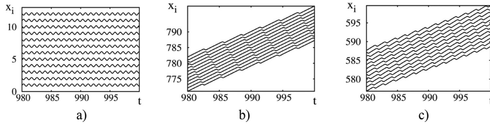
Fig. 1. According to the main text, here appear trajectories of N=12 active units in an one-dimensional lattice with excited (a) optical mode (6,6), (b) one-soliton mode (11,1), (c) two-soliton mode (10,2).
