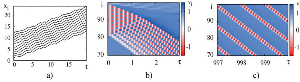
Fig. 2. Trajectories of active particles in an one-dimensional lattice with excited a) cluster of dissipative solitons (two solitons moving close to each other), b) fragment of the optical mode evolving fast to a cluster of 9 solitons, c) multi (9)-soliton mode.
