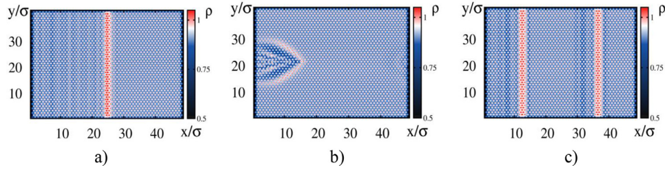
Fig. 5. Crystal-like triangular lattice. Metastable states: plane soliton a), soliton excited in a single rod b), two plane solitons c). All solitons propagate along the x -axis. Parameter values: b\sigma = 5 , d = 1.35\sigma and \nu = 0.035\sigma .
