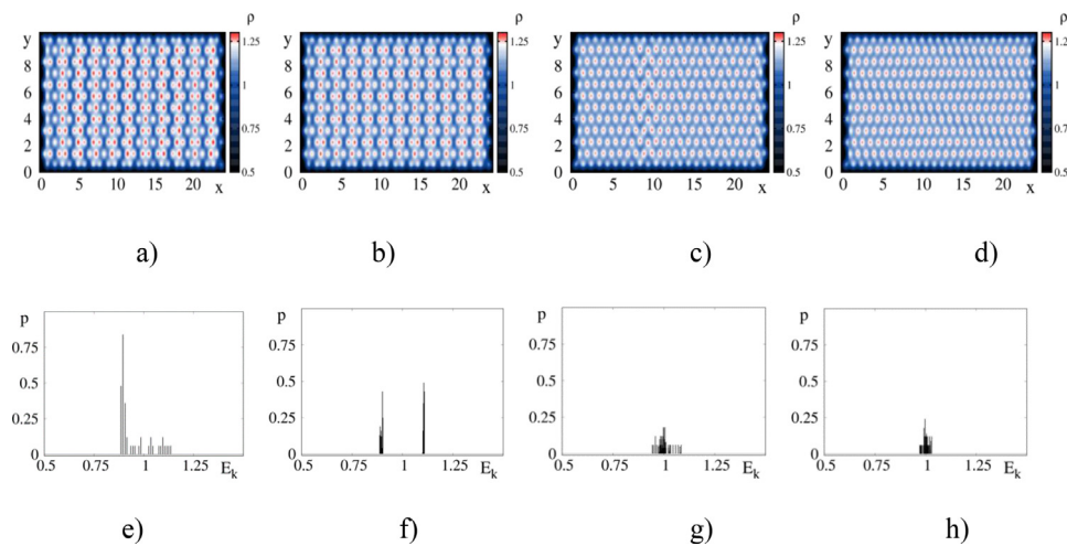
Fig. 9. Crystal-like triangular lattice. Translational mode after noise influence (from left to right – with different realizations of noise). Top panels: a)-d) spatial distribution of particles. Bottom panels: e)-h) kinetic energy distribution. Average translation velocity is along the OY axis. Parameter values: b\sigma = 5 , \mu = 7 , D_n = 0.5 , \tau_n = 350 .
