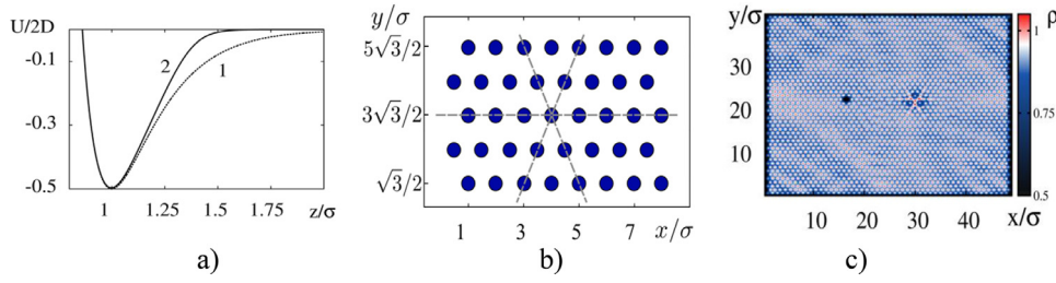
Fig. 4. Crystal-like triangular lattice. a): profiles of the standart (line 1) and modified (line 2) Morse potentials with parameter values b\sigma = 5 , d = 1.35\sigma and v = 0.035\sigma . b): schematic representation of a lattice with triangular symmetry; lines show the crystallographic axes. c): a steady state of a lattice with two defects: a vacancy at (17; 23) and interstitial particle at (30; 23).
