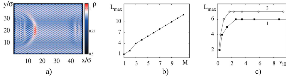
Fig. 6. Crystal-like triangular lattice. Horseshoe-like shape soliton, initially embracing M = 15 units (a) and dependence of maximal track lengths on the width of the plane horseshoe-like shape soliton front M in a lattice with b\sigma = 5 , \mu = 1.41 , v_0 = 0.14\omega_c\sigma (b); dependence of maximal track lengths on the initial particle velocity for b\sigma = 4 (line 1) and b\sigma = 6 (line 2), \mu = 1.41 (c).
