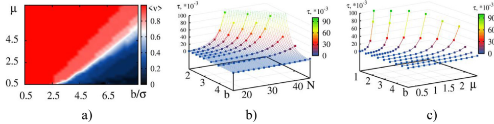
Fig. 3. Regions of realization of modes with different average velocity of units in the parametric plane $(b\sigma, \mu)$ a); dependence of transient time on the potential stiffness, $b\sigma$, in one-dimensional lattices with different number of particles $N$ for $\mu = 1$, b) and for varying values of $\mu$ with $N = 20$.
