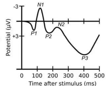
Event-Related Potential
