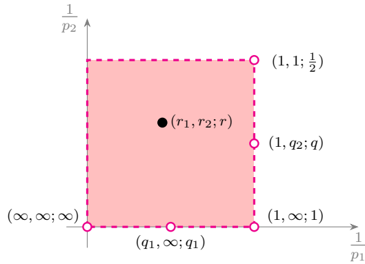
Figure 5.2: Theorem 5.0.3.
