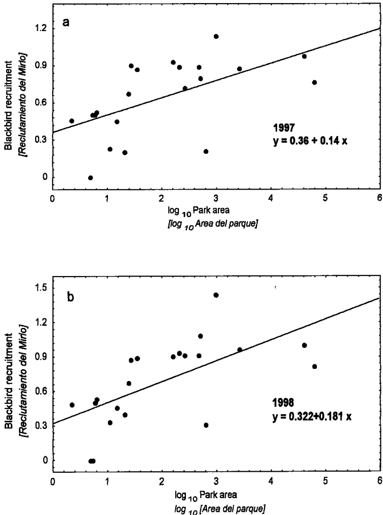
FIG. 2.—Relationship between Blackbird ( Turdus merula ) recruitment and patch area (ha) in 21 urban parks of the city of Madrid (Spain) in two consecutive breeding seasons, 1997 (a) and 1998 (b). In both years the linear regression models yielded significant relationships (1997, F_{1,19} = 9.12 , R^2 = 0.29 , P < 0.01 ; 1998, F_{1,19} = 12.14 , P < 0.01 , R^2 = 0.36 ).
