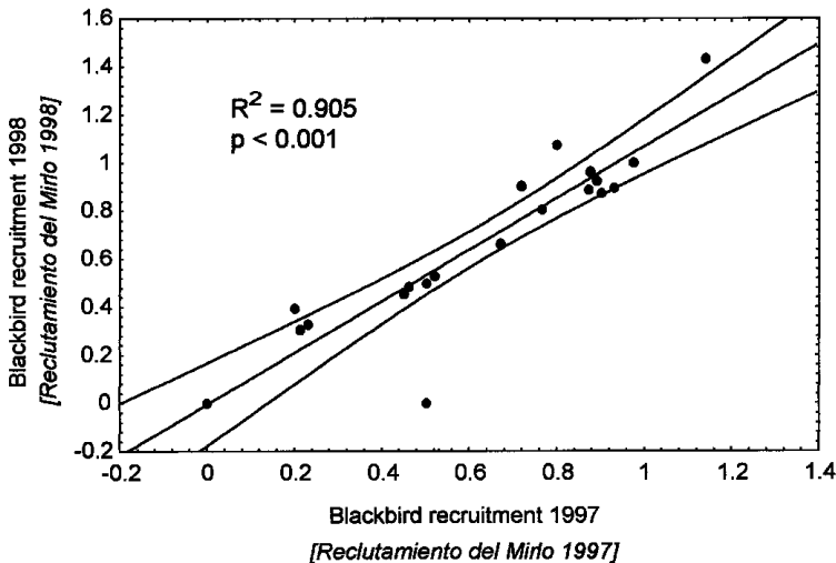
FIG. 1.—Spatial and temporal constancy of Blackbird ( Turdus merula ) recruitment patterns in 21 urban parks of Madrid (Spain). The graph shows the correlation between 1998 and 1997 recruitment values for each park with the 95% confidence intervals for such correlation.
