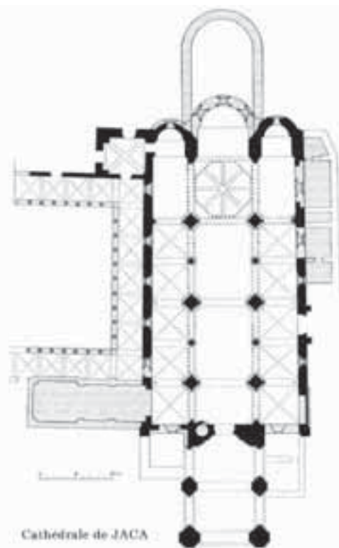
Fig. 5. Plan, Jaca cathedral. A. CANELLAS LÓPEZ and A. SAN VICENTE, Aragon roman , La Pierre-qui-Vire, 1971, p. 154.
