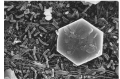
Mesophilic bacteria Acidithiobacillus surrounding a molybdenite crystal.
