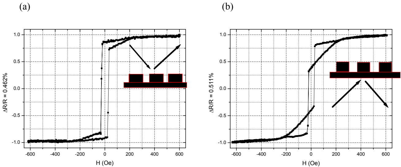
Figure 1: Hysteresis loops for a structure consisting of a continuous Co film with an array of Co stripes on top when the light is shined from (a) the patterned side, and (b) the flat side. The insets show the magneto optical measurement configuration (see text)
