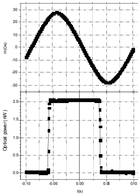
Figure 2: Applied field and variation of the diffracted light at an angular position corresponding to the stripe array periodicity when light is shined from the flat side of the structure.
