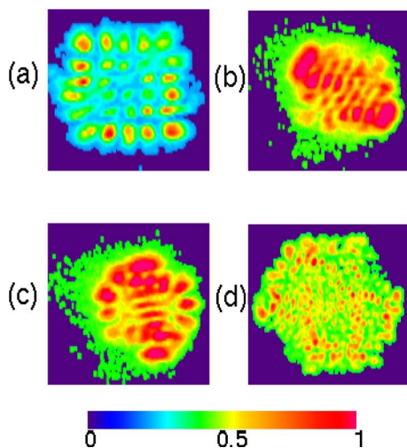
Fig. 1. (Color online) Instantaneous intensity patterns (resolution time 9 ns) for pumping 2.7 times above threshold: (a)–(c) for 4 \mu\text{s} of time delay from the beginning of the pulse, (d) for 40 \mu\text{s} of delay. Pattern size 6 mm \times 6 mm, approximately.
