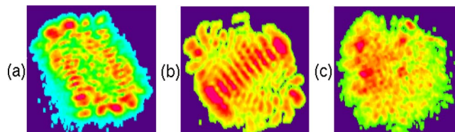
Fig. 2. (Color online) Instantaneous intensity patterns (resolution time 3 ns) for pumping 4 times above threshold (a), (b) for 8 \mu\text{s} of time delay from the beginning of the pulse, (c) for 23 \mu\text{s} of delay. Pattern size 6 mm \times 6 mm, approximately.
