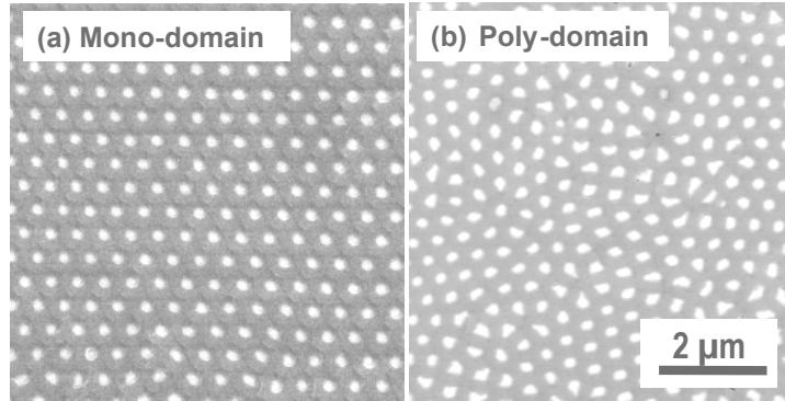
Fig 2: Nickel filled alumina templates fabricated via imprint lithography (a) and via self-ordering (b) .
