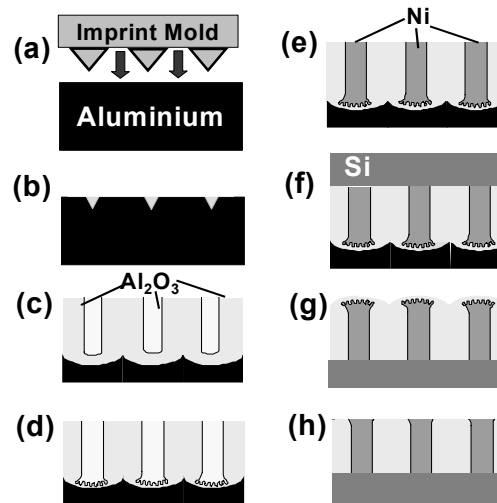
Fig. 1: Preparation steps for fabrication nickel nanowire arrays embedded in an alumina matrix and fixed to a Si substrate via imprint lithography.
