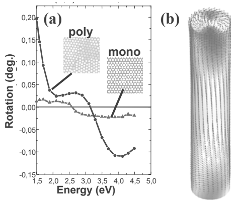
Fig. 3: (a) Magneto-optical spectra of 500 nm-period Ni nanowire array with 2D-poly- and monocrystalline arrangement in two dimensions. (b) Micromagnetic simulation of the magnetization for a single Ni nanowire with a diameter of 180 nm and a length of 5 \mu\text{m} .
