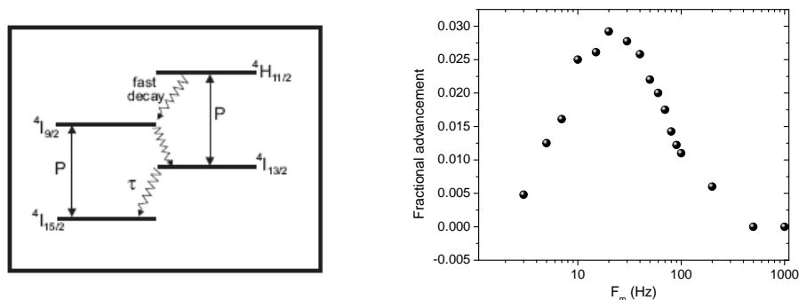
Fig. 1. Left: \text{Er}^{3+} ions energy levels, coupled by a 787 nm laser beam. Right: Fractional advancement measured for sinusoidal signals with different modulation frequencies, measured on a 1 m-long EDF with \text{Er}^{3+} ions density of 2,7 \times 10^{25} .
