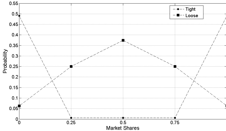
Figure 2: Invariant distribution of annual market shares (one year equals four periods).
