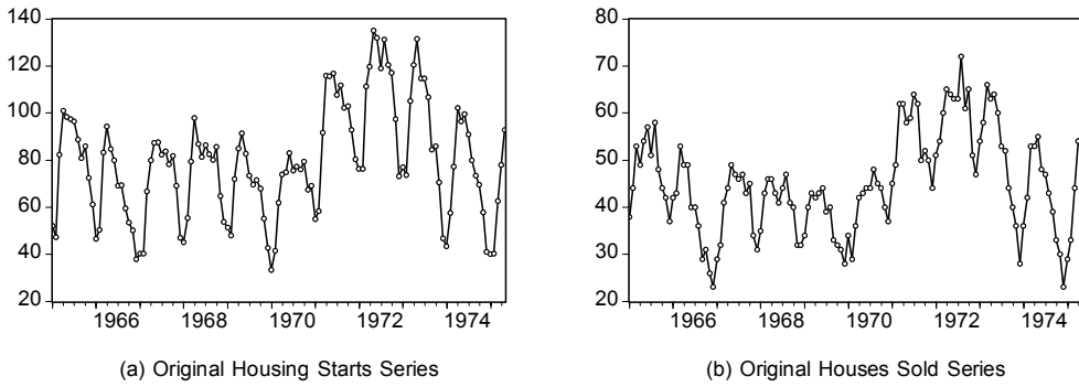
Figure A1. The Original (Seasonally Unadjusted) Census Housing Data (in thousands) over the Period January 1965 Through May 1975.
