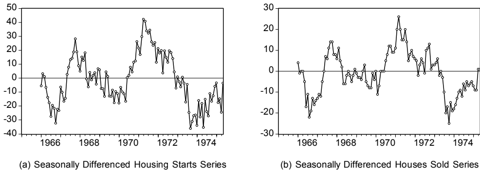
Figure A2. The Seasonally Differenced Census Housing Data (in thousands) over the Period January 1966 Through May 1975.
