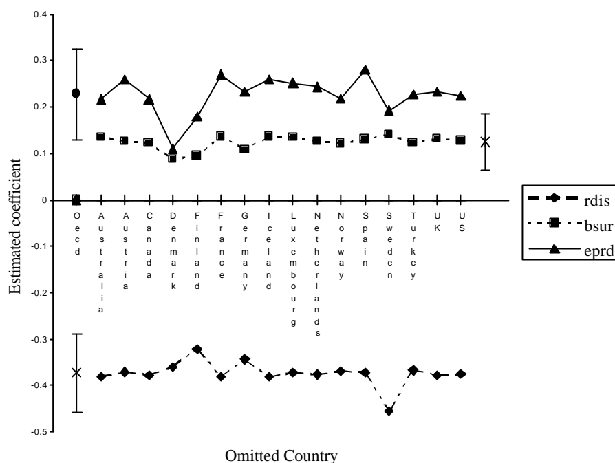
Figure 1 Testing Parameter Homogeneity
