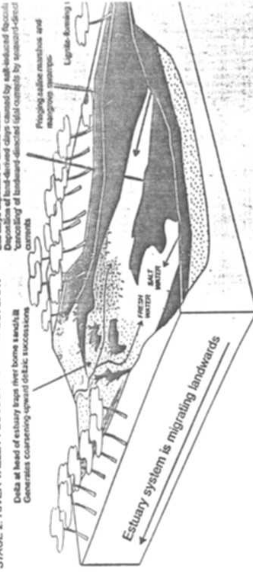
STAGE 2. RIVER VALLEY FLOODED TO FORM ESTUARY
