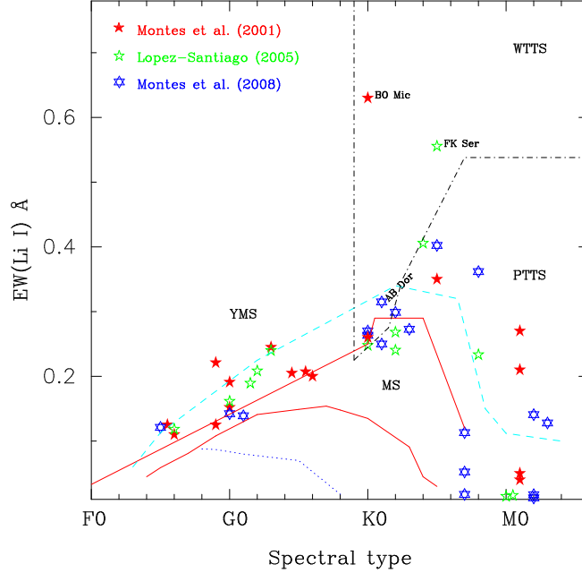
Fig. 1 Equivalent width of the Li I line at 6707.8 Å (from [7]; [8]; [1]; [9]), as a function of spectral type for the selected stars, compared with the envelopes of well-known stellar clusters (ages from 10 to 600 Myr). The dot-dashed lines represent the T_{\text{eff}} cutoff at 5250 K and the Li isoabundance line for \log N(\text{Li}) = 2.8 (minimum abundance for TTS) used in the PTTS spectroscopic definition by [4].
