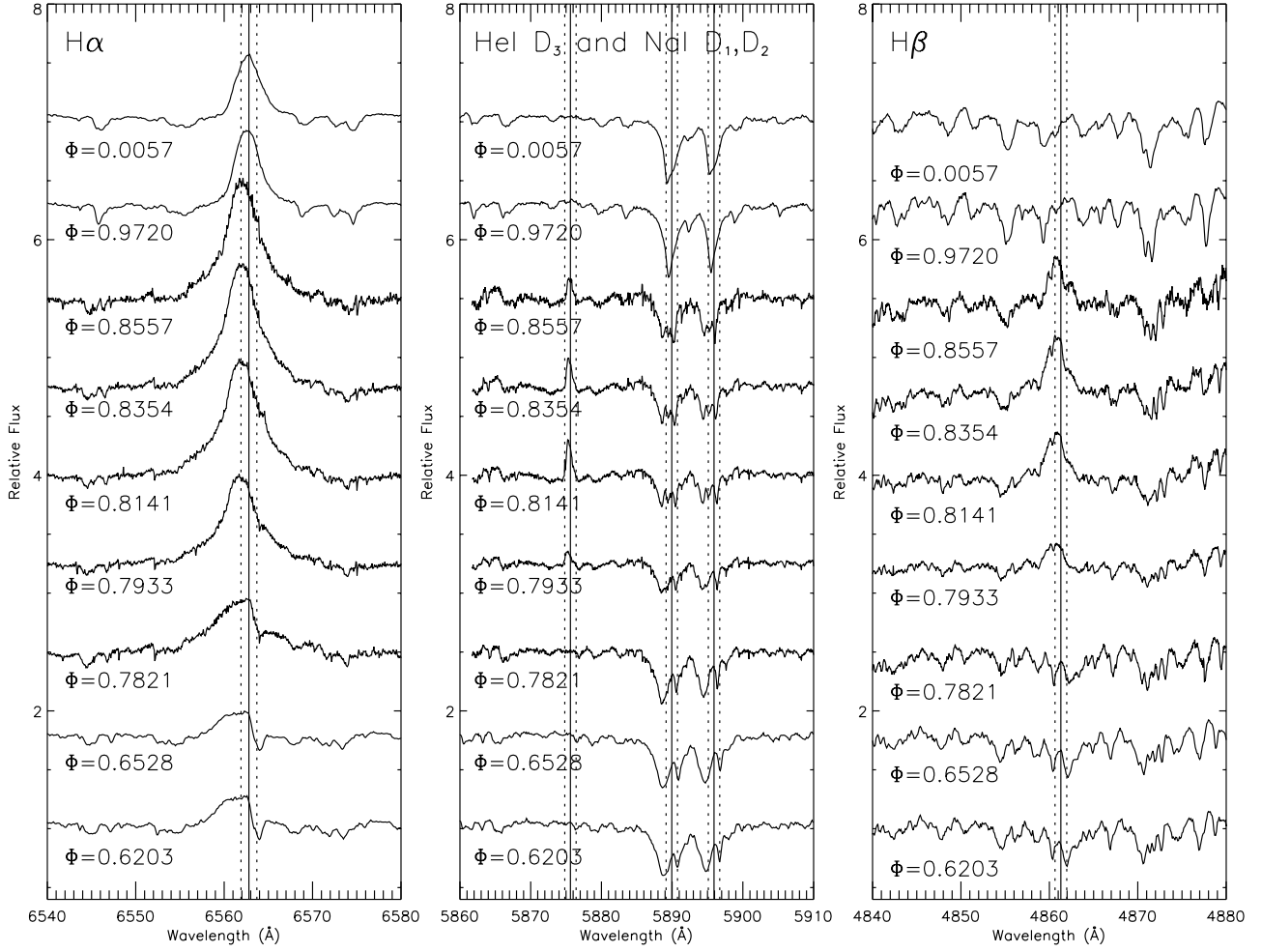
Fig. 11. The observed spectra for H\alpha (left panel), He\ I\ D_3 and Na\ I\ D_1, D_2 doublet (middle panel) and H\beta (right panel) of the second monitored flare starting at JD 2451151.07 arranged in order of the orbital phase. The vertical lines correspond to the rest wavelength of the lines (solid line) and the corresponding maximum rotational broadening of the K1 IV component of v \sin i = \pm 41\text{ km s}^{-1} (dotted line), respectively.
