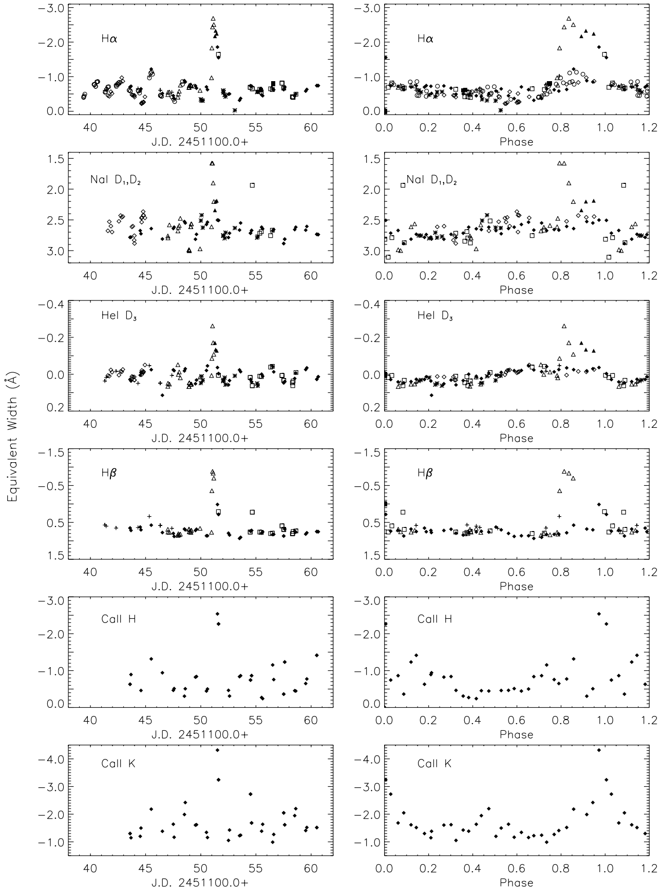
Fig. 9. The equivalent width as a function of Julian date and as a function of phase for H\alpha , Na I D_1, D_2 doublet, He I D_3 , H\beta and Ca II H & K lines observed at the different sites, namely: OHP152 (open circle), OHP193 (+), KPNO (open diamond), ESO (filled diamond), Mt. Stromlo (open triangle), Xinglong (*), INT (open square), LNA (filled square) and SAAO (filled triangle).
